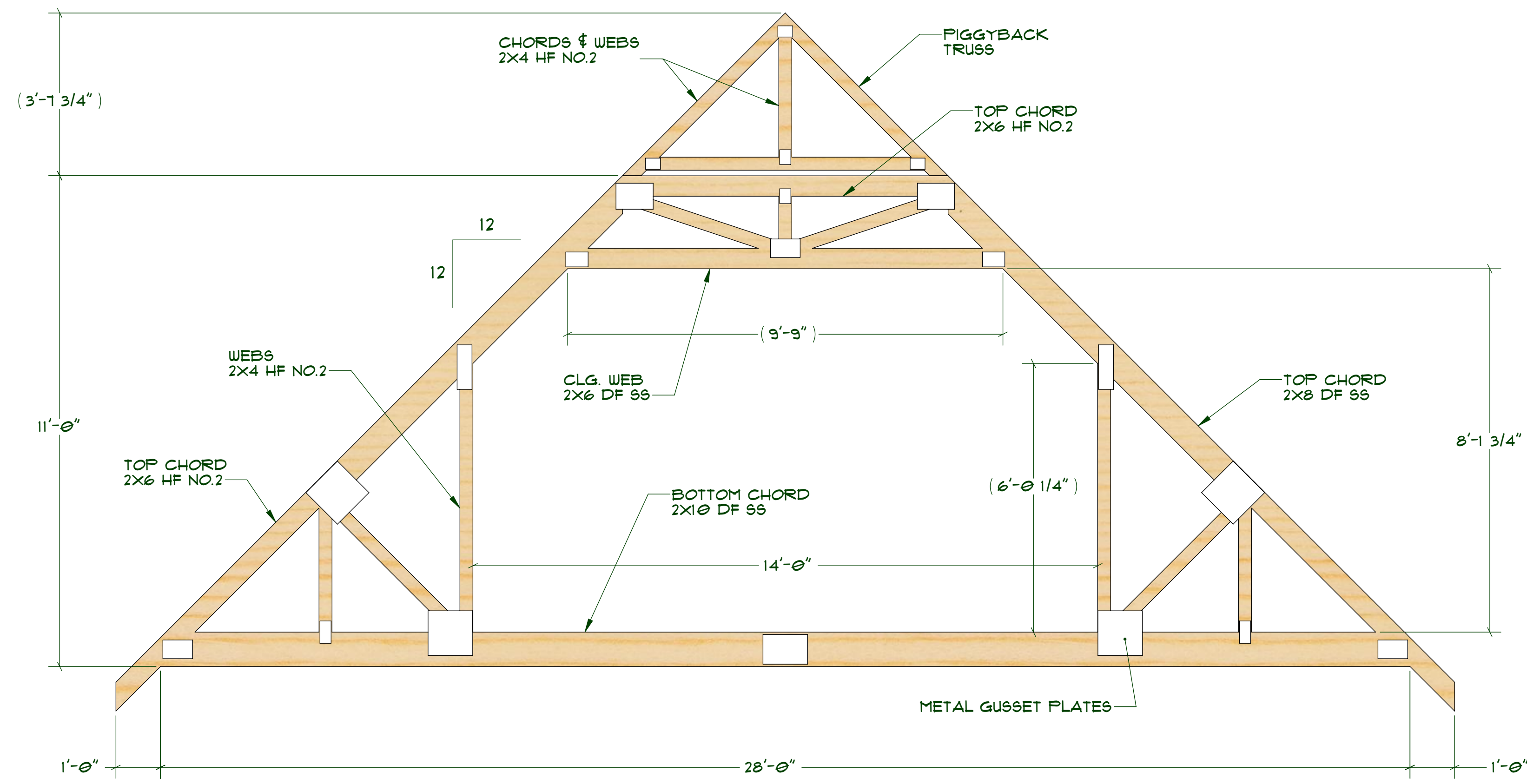
28' ATTIC TRUSS W/ PIGGYBACK
